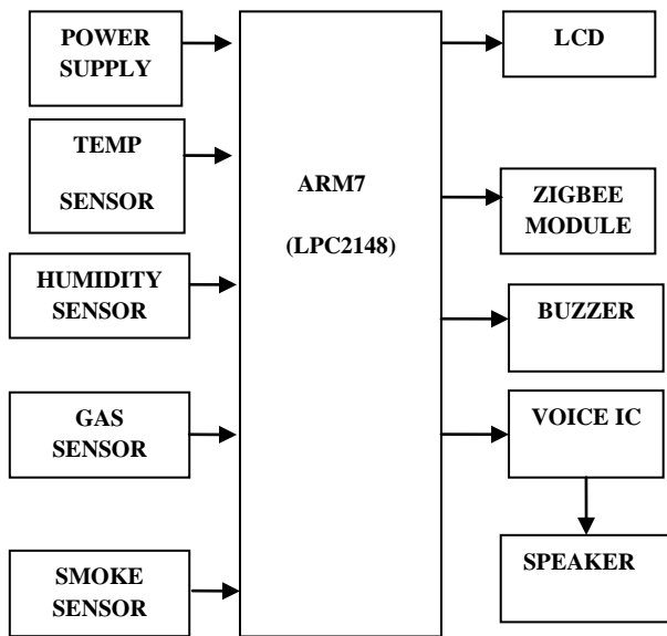
Fig.1.Blockdiagram
