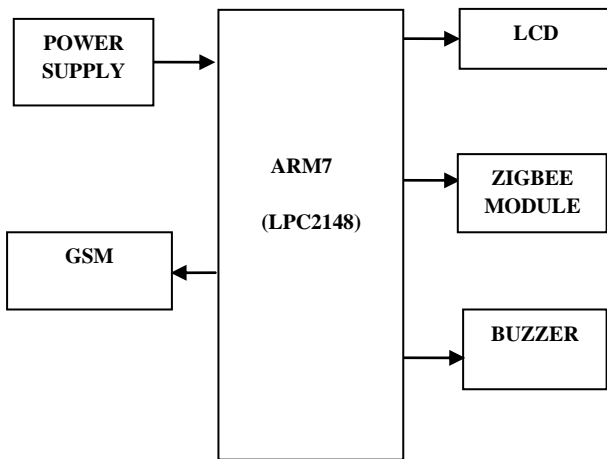
Fig.2.Block diagram
